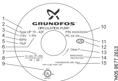
Fig. 1 Nameplate
