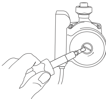
Fig. 2 Rotating the shaft by hand
